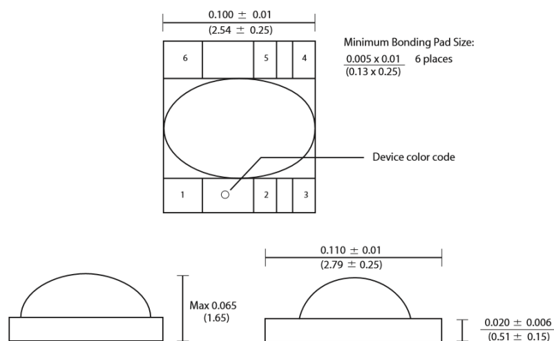
Figure 2. IBI500 Package Dimensions
