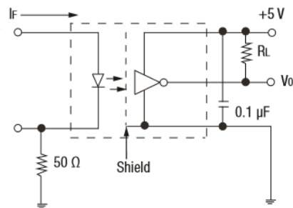
Figure 7. IBI500 Switching Test Circuit
