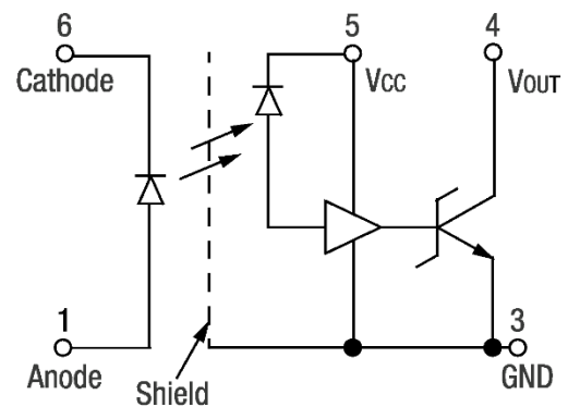
Figure 1. IBI500 Schematic Diagram
