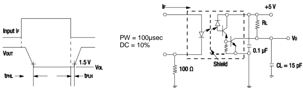
Figure 6. IBI400 Switching Test Circuit
