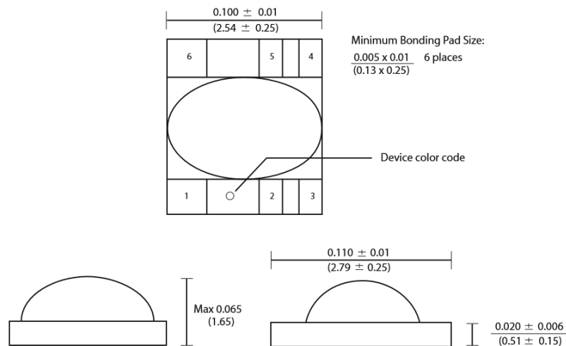
Figure 2. IBI400 Package Dimensions
