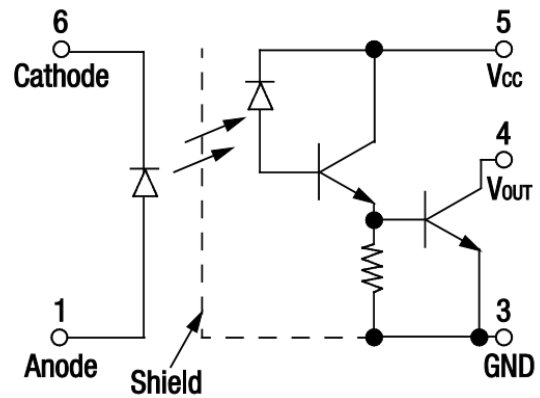
Figure 1. IBI400 Schematic Diagram
